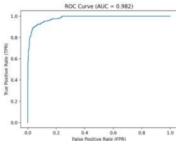
Equation 1: Derive TPR (Recall) step-by-step
